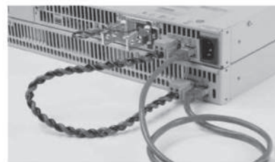
Figure 7. N7909A power dissipater unit rear connections to a 1 kW APS power supply
