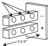
Bus Bar Detail 3/8" Diameter (6)
