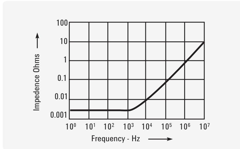
Typical output impedance of a constant voltage power supply
