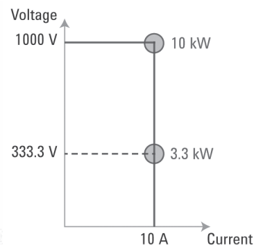
Figure 2. Rectangular output characteristic
