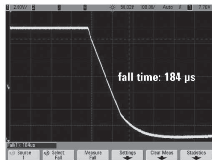
Figure 5. Pulse fall time of < 200 \mu s
