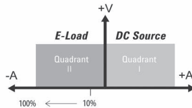
Figure 2. Adding N7909A power dissipater units to an APS supply extends its ability to sink current from 10% to 100% of its rated current
