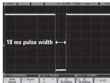
Figure 4. Voltage interrupt pulse
