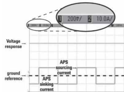
Figure 3. Shows an example of an APS power supply smoothly pulsing back and forth from sinking current at -10 A to sourcing current at 10 A. The voltage level captured at high resolution on the top trace remains constant with no glitches.
