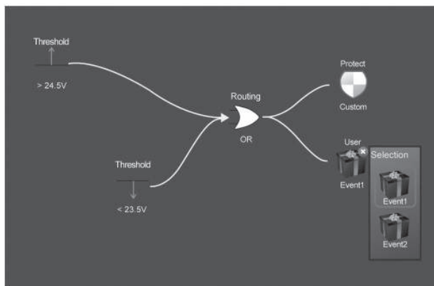
Figure 10. Configuring a trigger expression with the N7906A Power Assistant software
