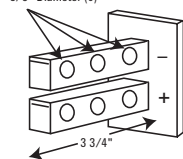
Buss Bar Detail 3/8" Diameter (6)
